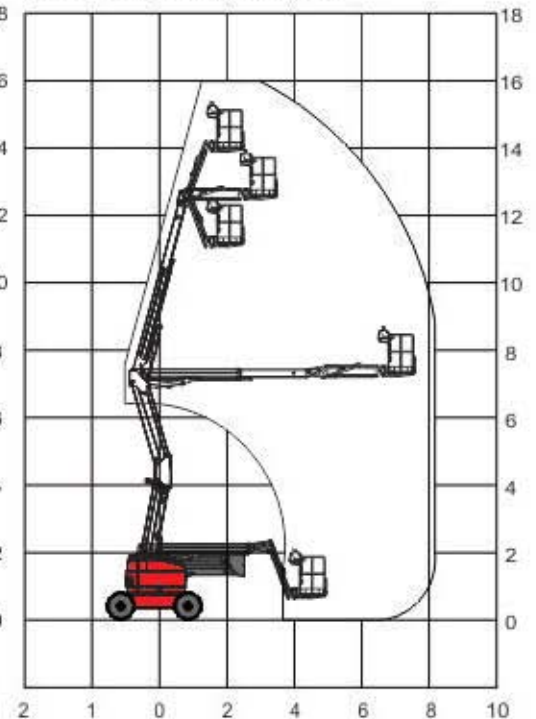
HZ160JRT Working Range
